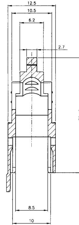
SECTION B-B
